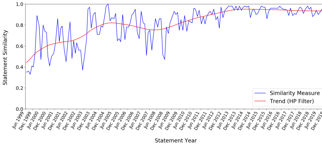
Figure 4: S^1 Statement Similarity with 1 statement lag
